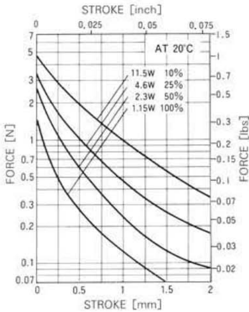
STROKE - FORCE
