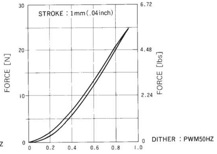
CURRENT [A] CURRENT - FORCE (TYPICAL)
